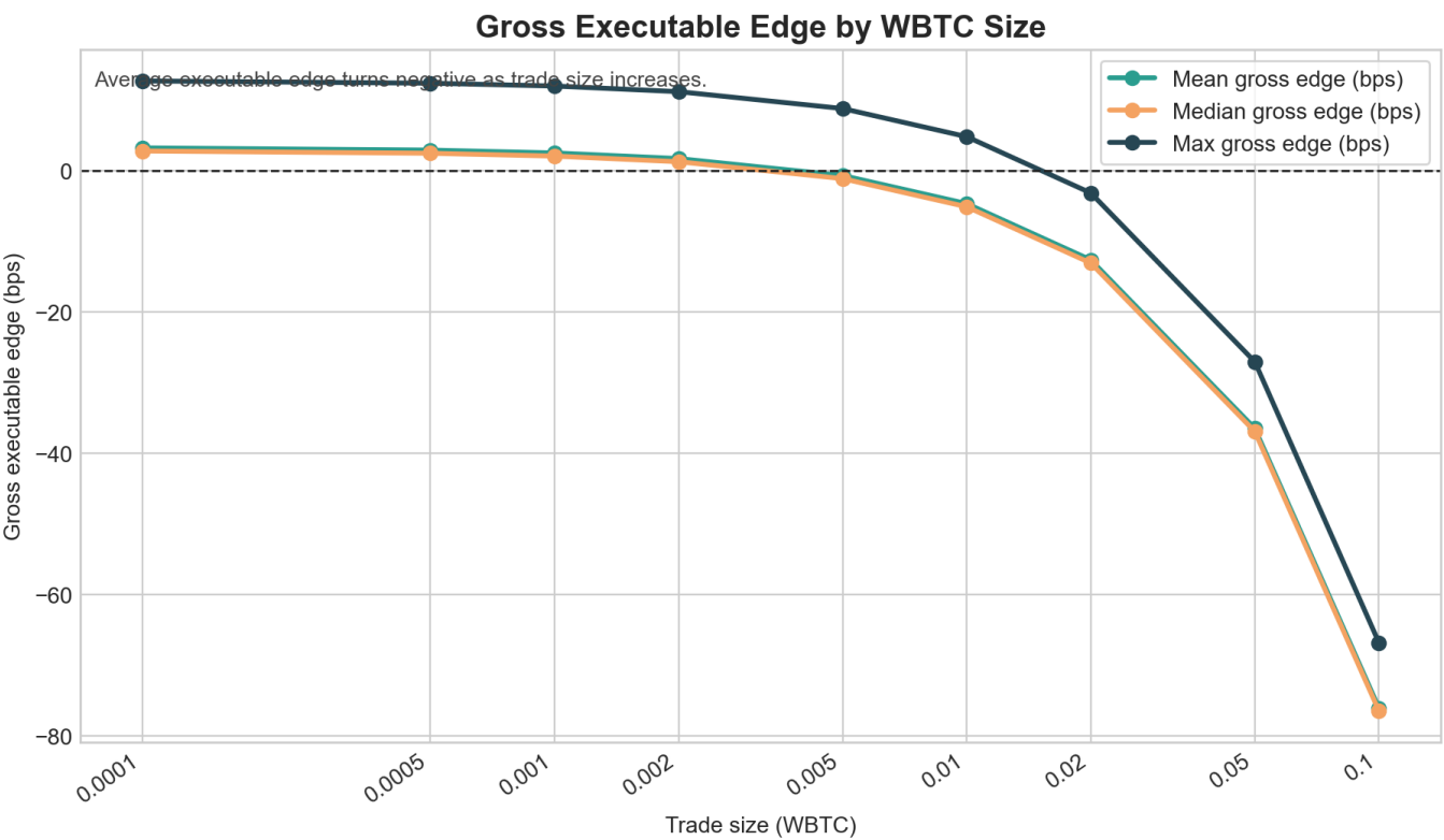
MEV Figure 4. Gross Executable Edge by WBTC Size
